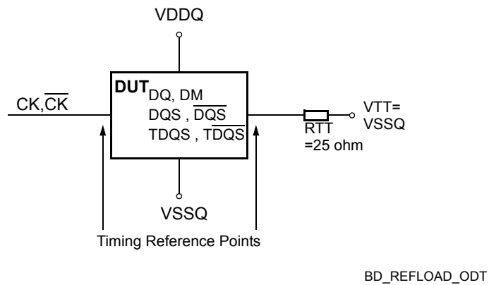
Figure 14. ODT Timing Reference Load
