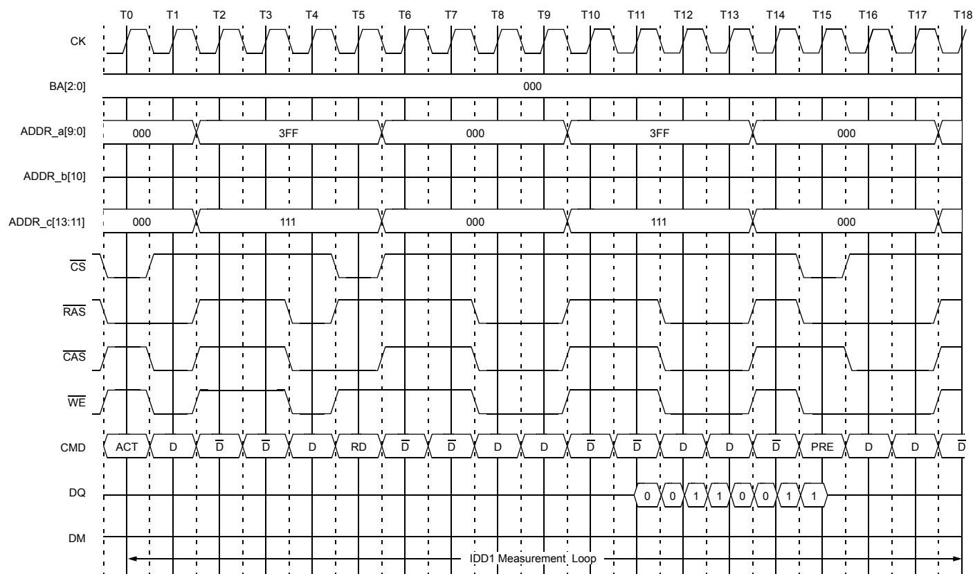
Figure 20. IDD1 Example (DDR3-800-666, 1Gb x8): Data DQ is shown but the output buffer should be switched off (per MR1 Bit A12 ="1") to achieve Iout = 0mA. Address inputs are split into 3 parts.
