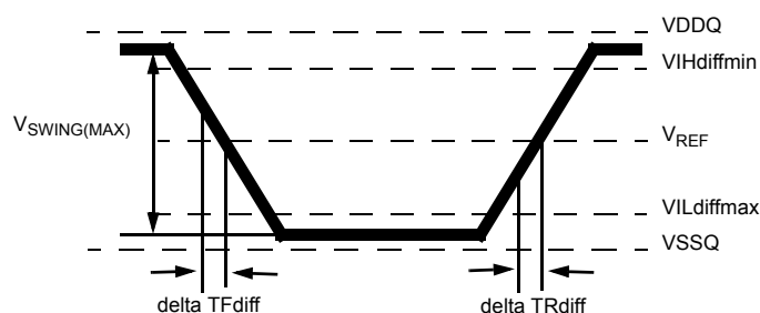
Figure 6. Differential Input Slew Rate definition for DQS, \overline{DQS} and CK, \overline{CK}
