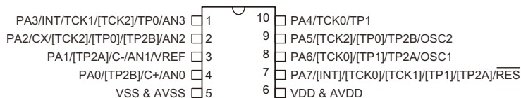
HT66F04 10 MSOP-A
