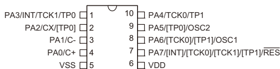
HT68F03/HT68F04 10 MSOP-A
