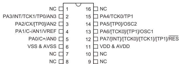
HT66F03 16 NSOP-A
