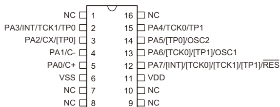
HT68F03/HT68F04 16 NSOP-A
