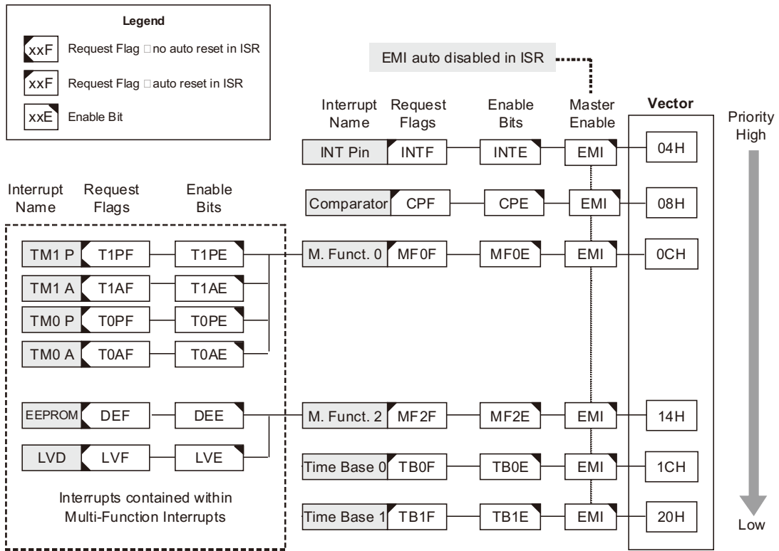
Interrupt Structure – HT68F03/HT68F04
