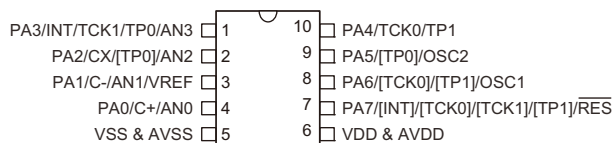
HT66F03 10 MSOP-A
