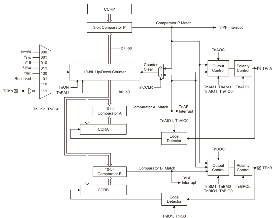
Enhanced Type TM Block Diagram
