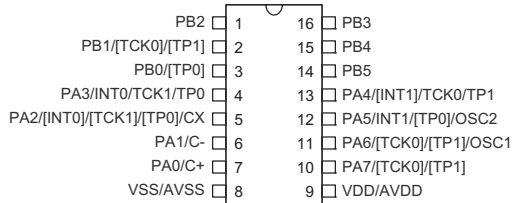
HT68F017 16 DIP-A/NSOP-A/SSOP-A
