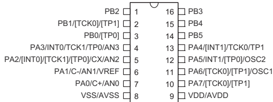
HT66F017 16 DIP-A/NSOP-A/SSOP-A
