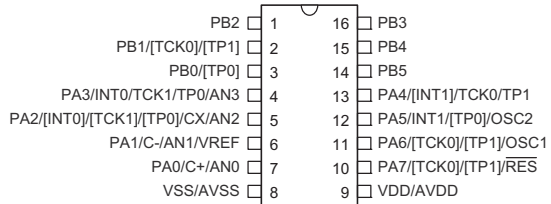
HT66F017R 16 DIP-B/NSOP-B/SSOP-B
