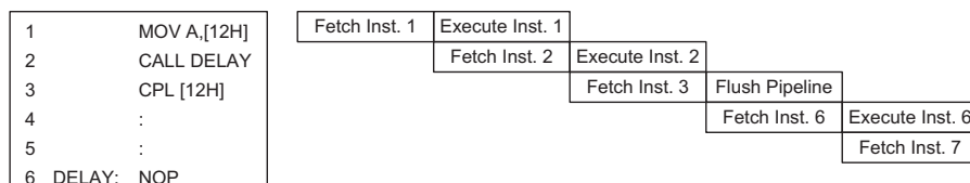
Instruction Fetching
