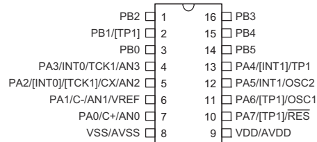
HT66F016R 16 DIP-B/NSOP-B/SSOP-B
