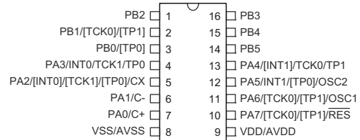
HT68F017R 16 DIP-B/NSOP-B/SSOP-B
