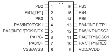
HT68F016R 16 DIP-B/NSOP-B/SSOP-B
